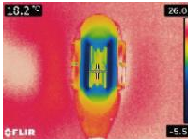
Cooling on both sides
